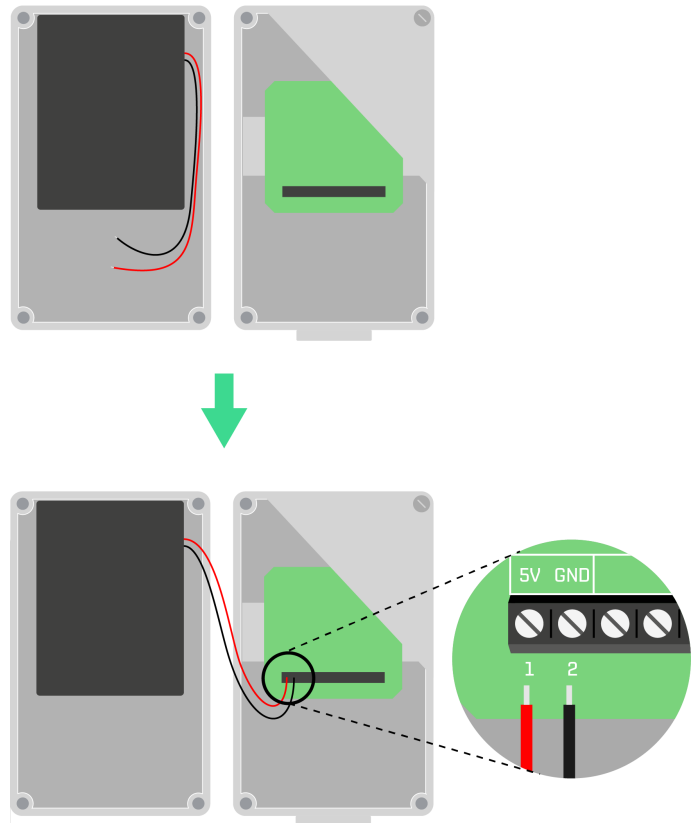
Rys. 3: Supply connection to the TCM SENSOR T
