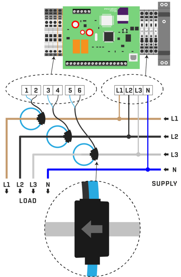
Fig. 1: Connection of Rogowski coils and power supply.
